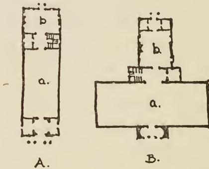
FIG. 22. A is a logical arrangement but unsuited to the position of the building on an important street. B is a better solution, but the rear portion of the building is still not absolutely correct in arrangement. a: The art gallery. b: The library.
